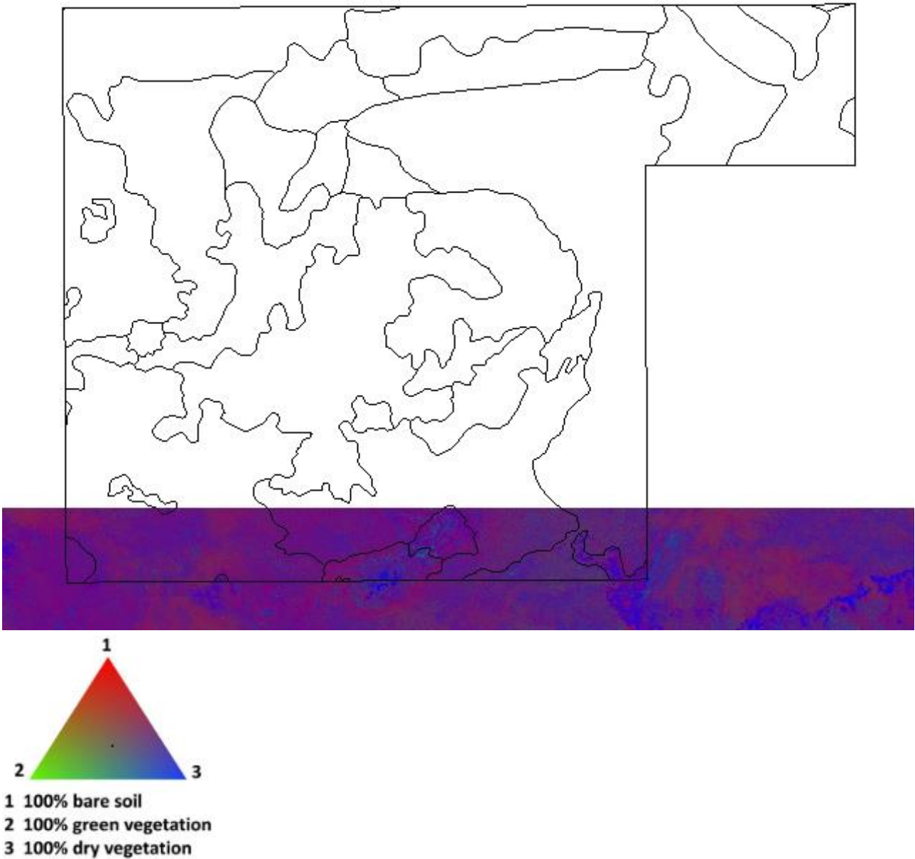
Figure 1 Estimated Fractional Cover Map
